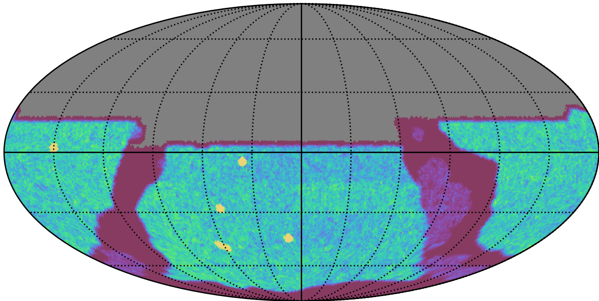
too_elab_r16_d3_gz_v3.4_10yrs All sky u band: NVisits
