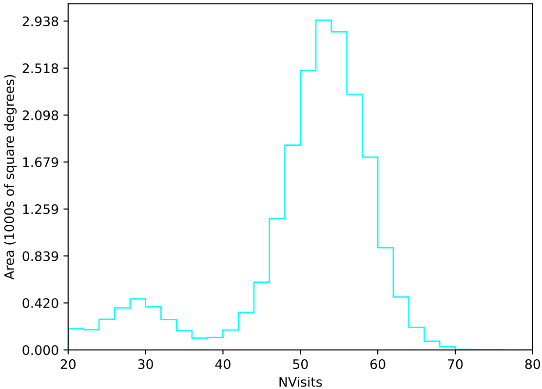
too_elab_r16_d3_gz_v3.4_10yrs All sky u band: NVisits
