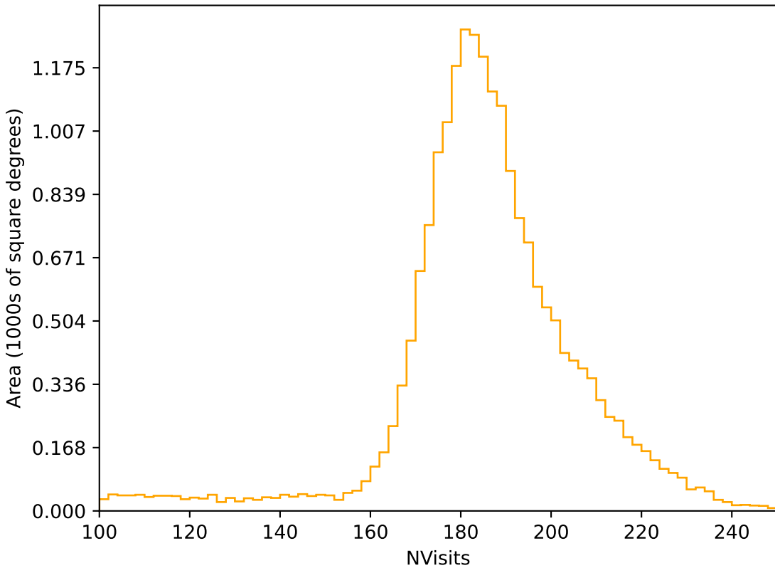
too_elab_r16_d3_gz_v3.4_10yrs All sky r band: NVisits
