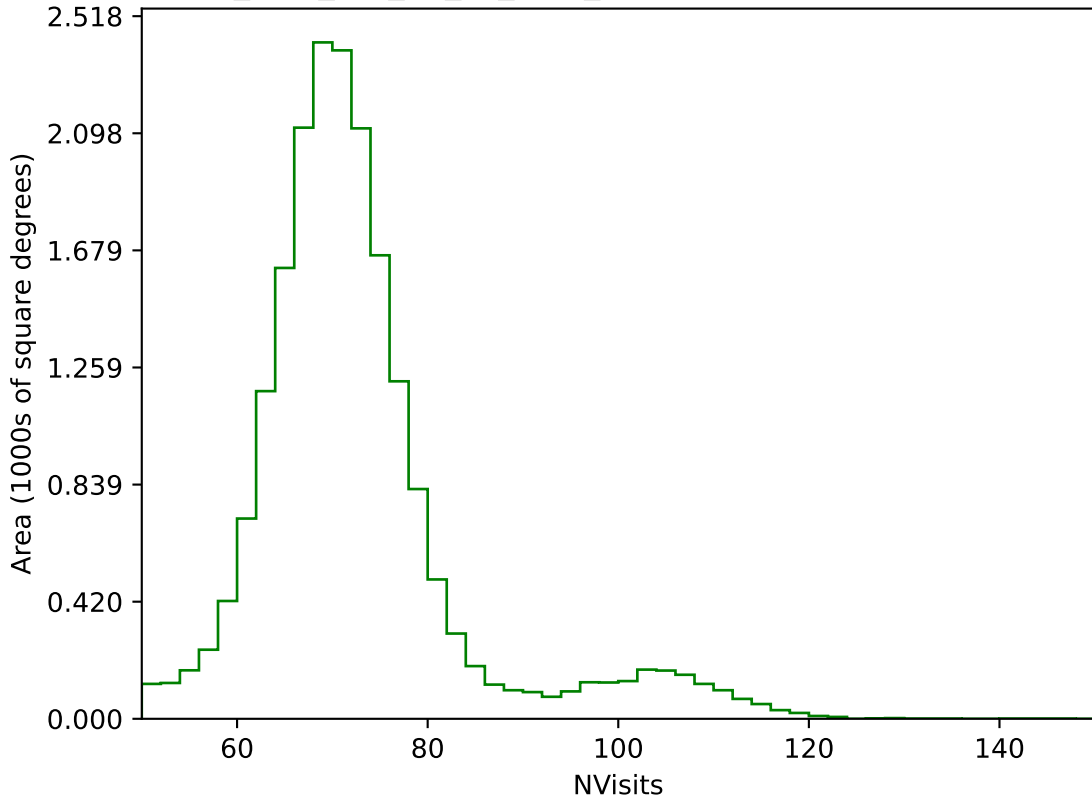
too_elab_r16_d3_gz_v3.4_10yrs All sky g band: NVisits
