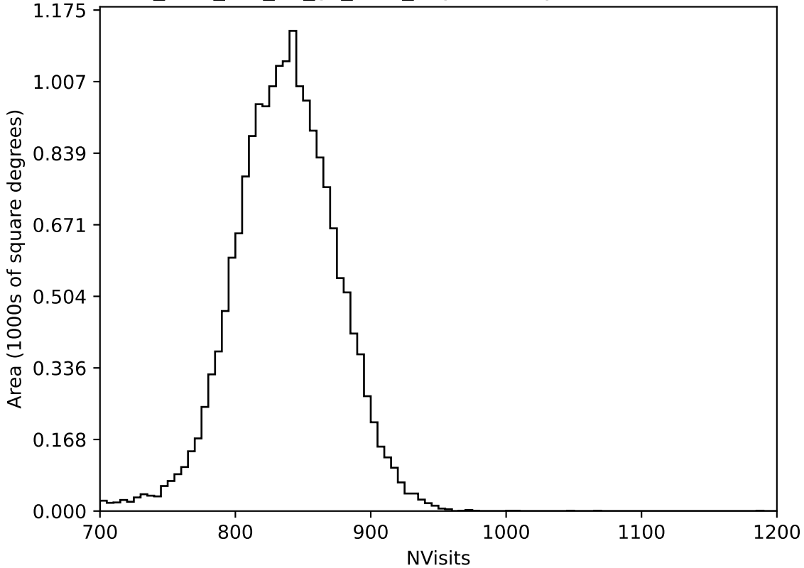
too_elab_r16_d3_gz_v3.4_10yrs All sky all bands: NVisits
