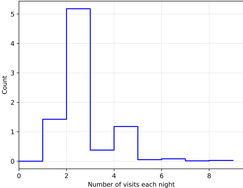
too_elab_r16_d3_gz_v3.4_10yrs WFD: NVisitsPerNight
