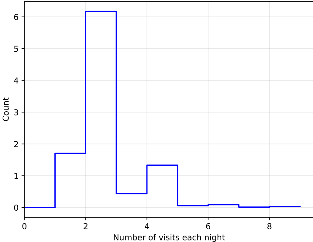
too_elab_r16_d3_gz_v3.4_10yrs All sky: NVisitsPerNight
