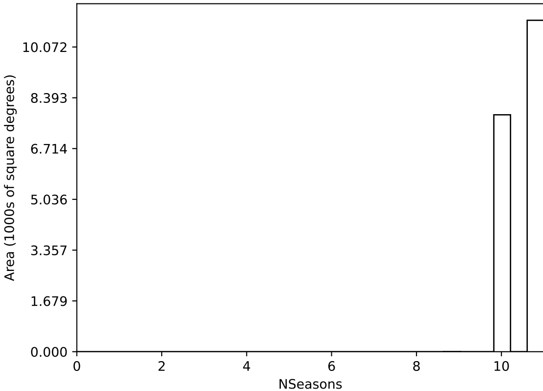
too_elab_r16_d3_gz_v3.4_10yrs WFD all bands: NSeasons
