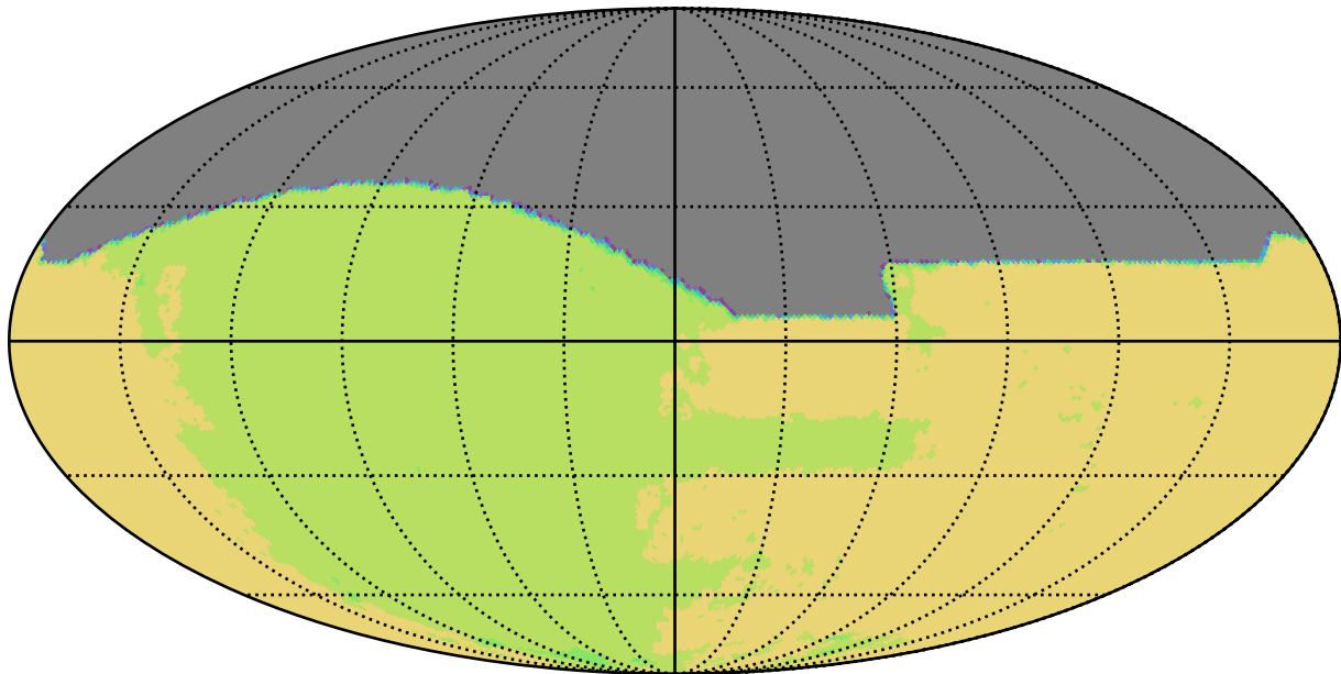
too_elab_r16_d3_gz_v3.4_10yrs All sky all bands: NSeasons
