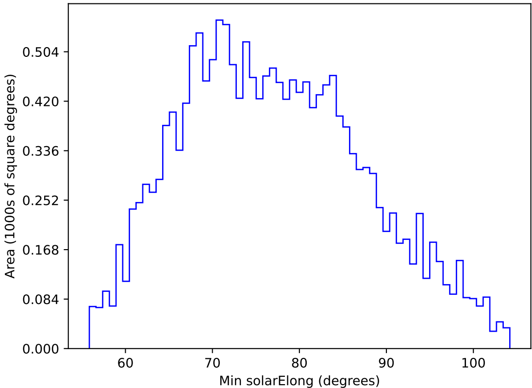
too_elab_r16_d3_gz_v3.4_10yrs WFD u band: Min solarElong
