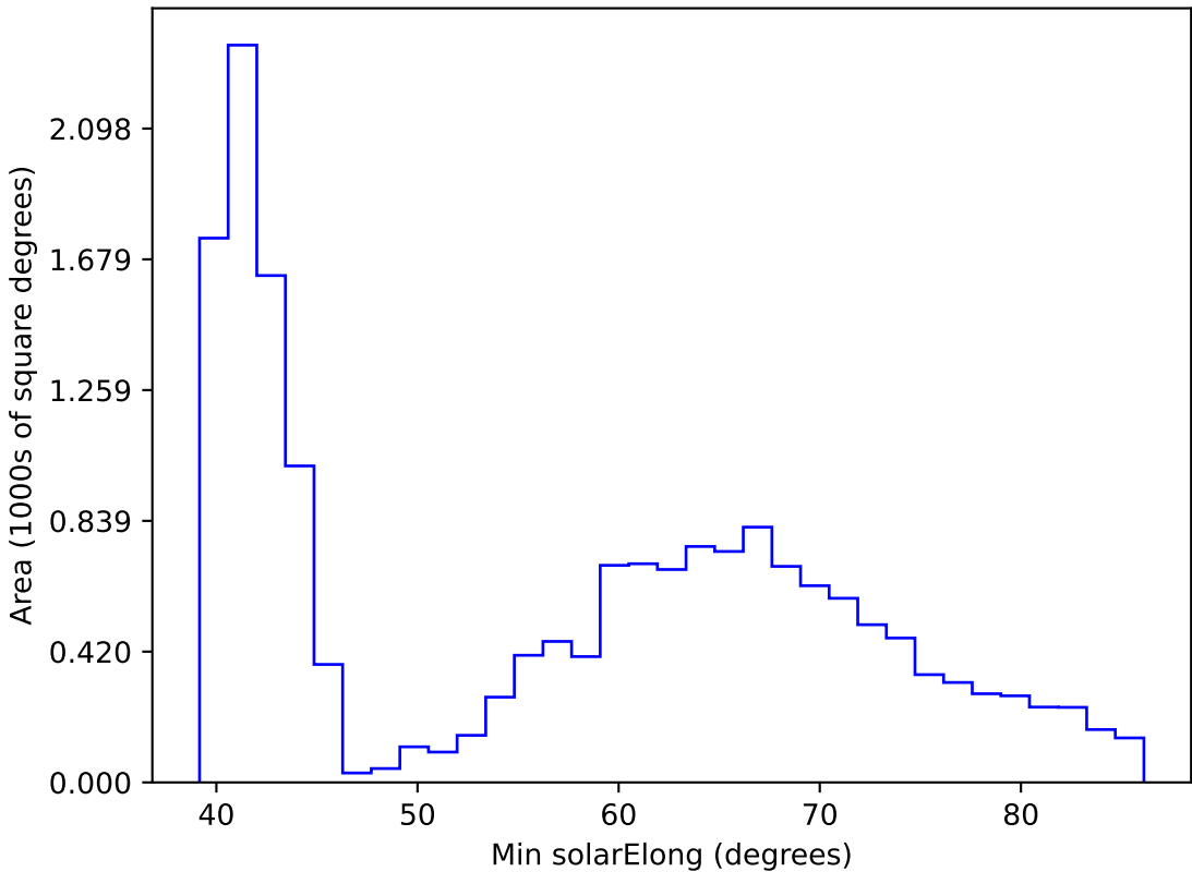
too_elab_r16_d3_gz_v3.4_10yrs WFD r band: Min solarElong
