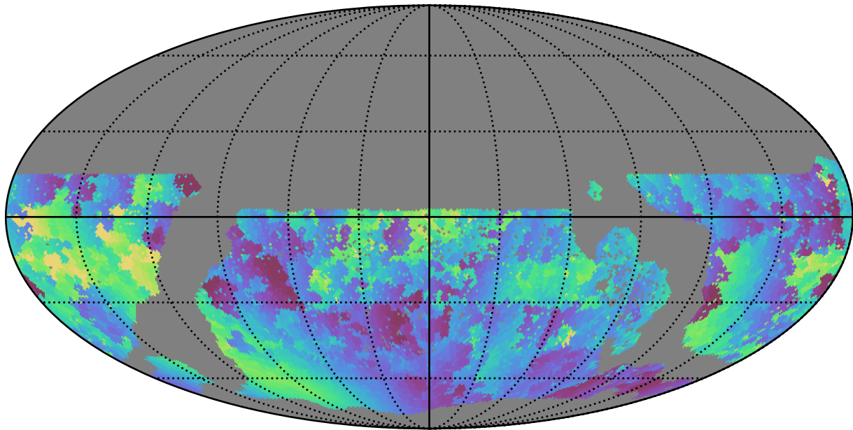
too_elab_r16_d3_gz_v3.4_10yrs WFD g band: Min solarElong
