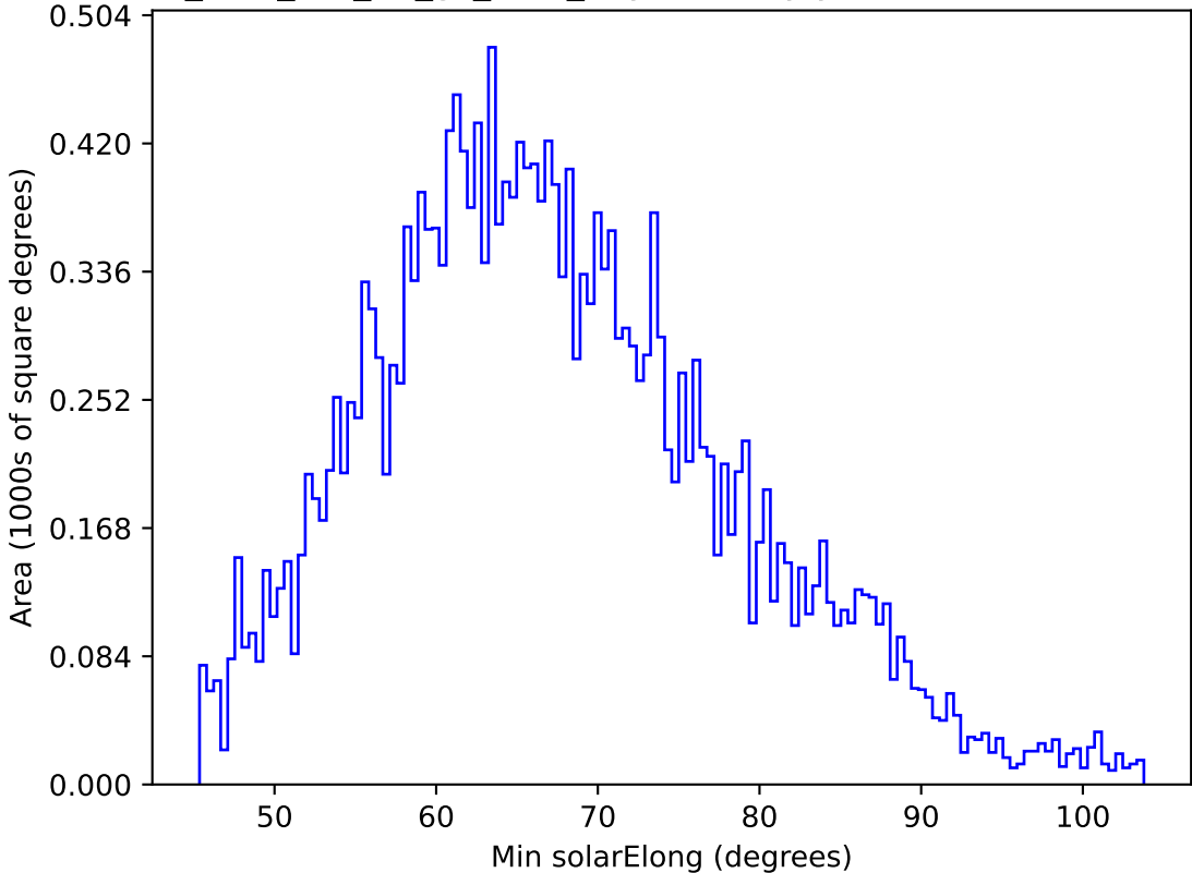
too_elab_r16_d3_gz_v3.4_10yrs All sky y band: Min solarElong
