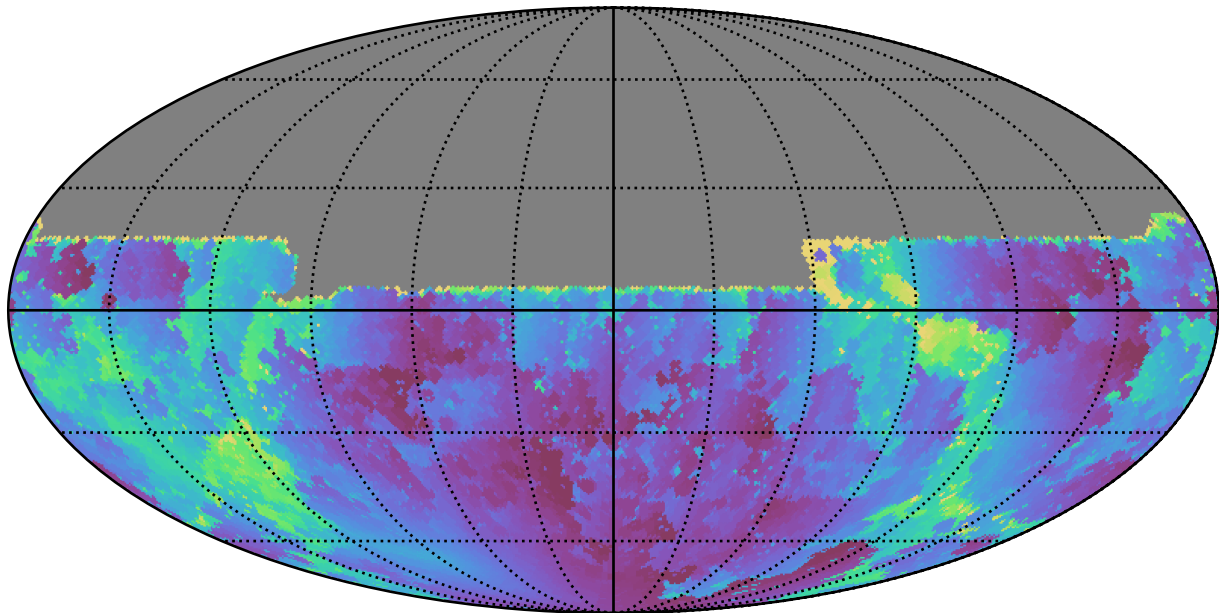
too_elab_r16_d3_gz_v3.4_10yrs All sky u band: Min solarElong
