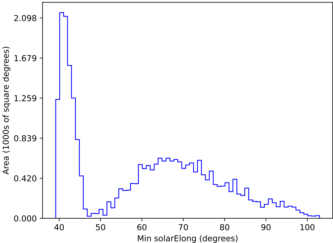
too_elab_r16_d3_gz_v3.4_10yrs All sky r band: Min solarElong
