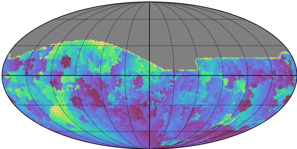
too_elab_r16_d3_gz_v3.4_10yrs All sky g band: Min solarElong
