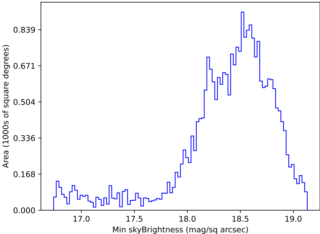
too_elab_r16_d3_gz_v3.4_10yrs Yr 1 z band: Min skyBrightness
