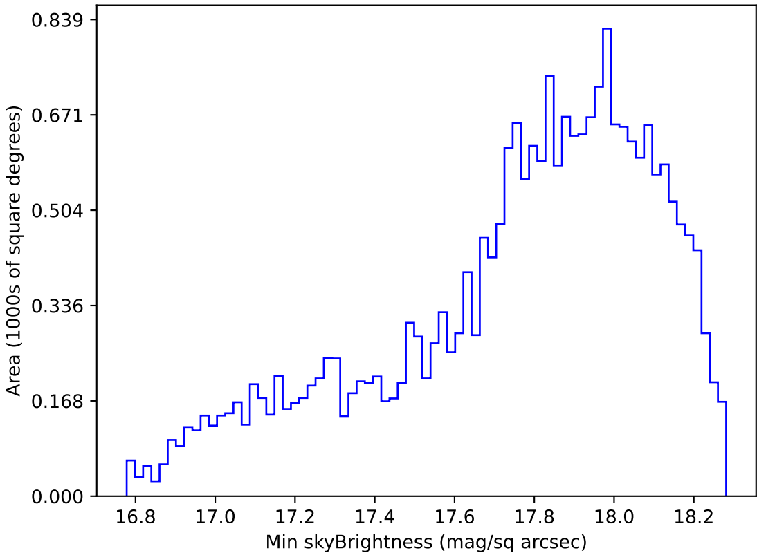
too_elab_r16_d3_gz_v3.4_10yrs Yr 1 y band: Min skyBrightness
