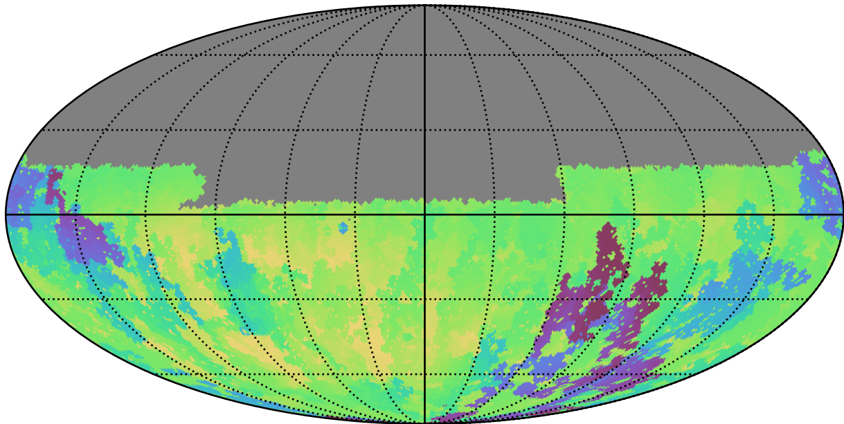
too_elab_r16_d3_gz_v3.4_10yrs Yr 1 u band: Min skyBrightness
