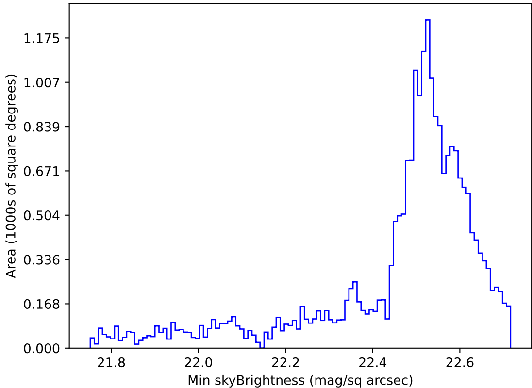
too_elab_r16_d3_gz_v3.4_10yrs Yr 1 u band: Min skyBrightness
