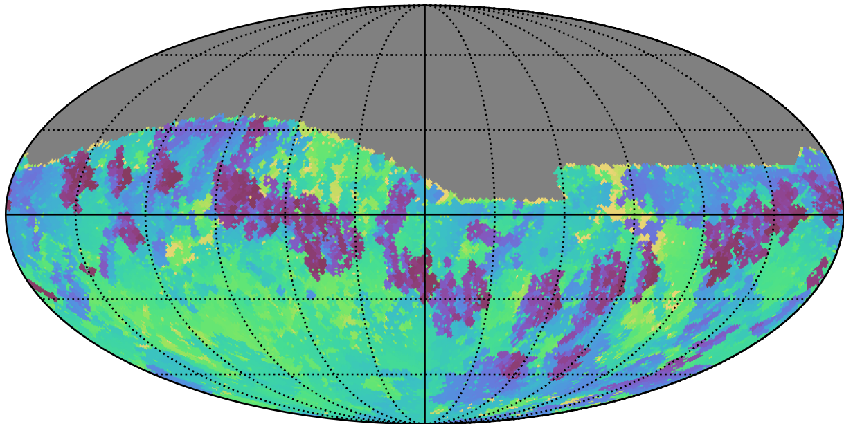
too_elab_r16_d3_gz_v3.4_10yrs Yr 1 i band: Min skyBrightness
