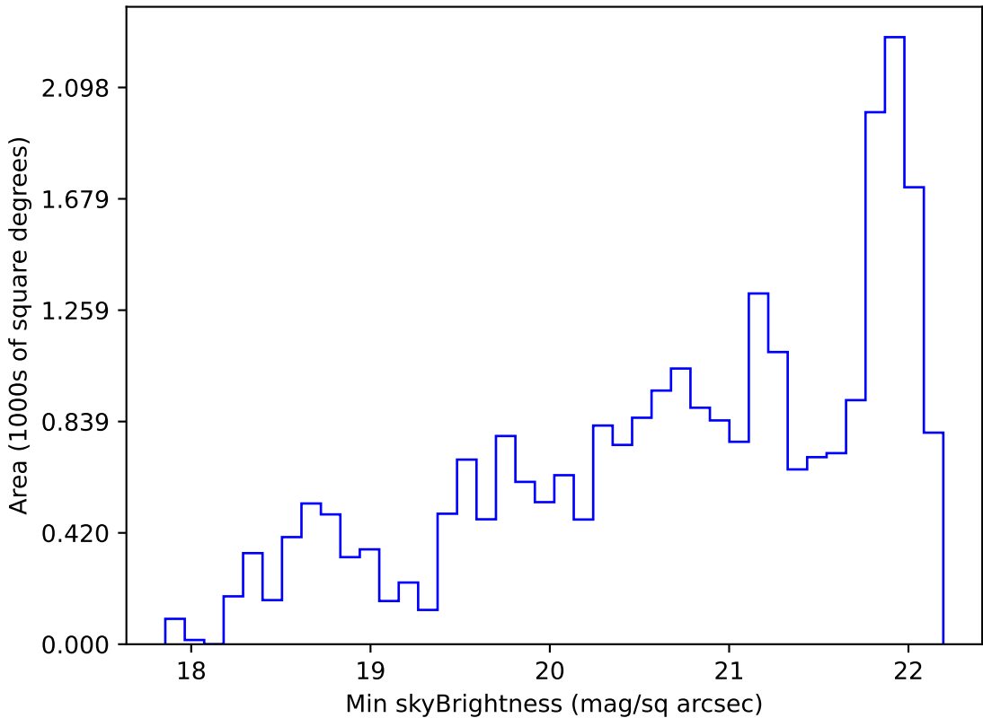
too_elab_r16_d3_gz_v3.4_10yrs Yr 1 g band: Min skyBrightness
