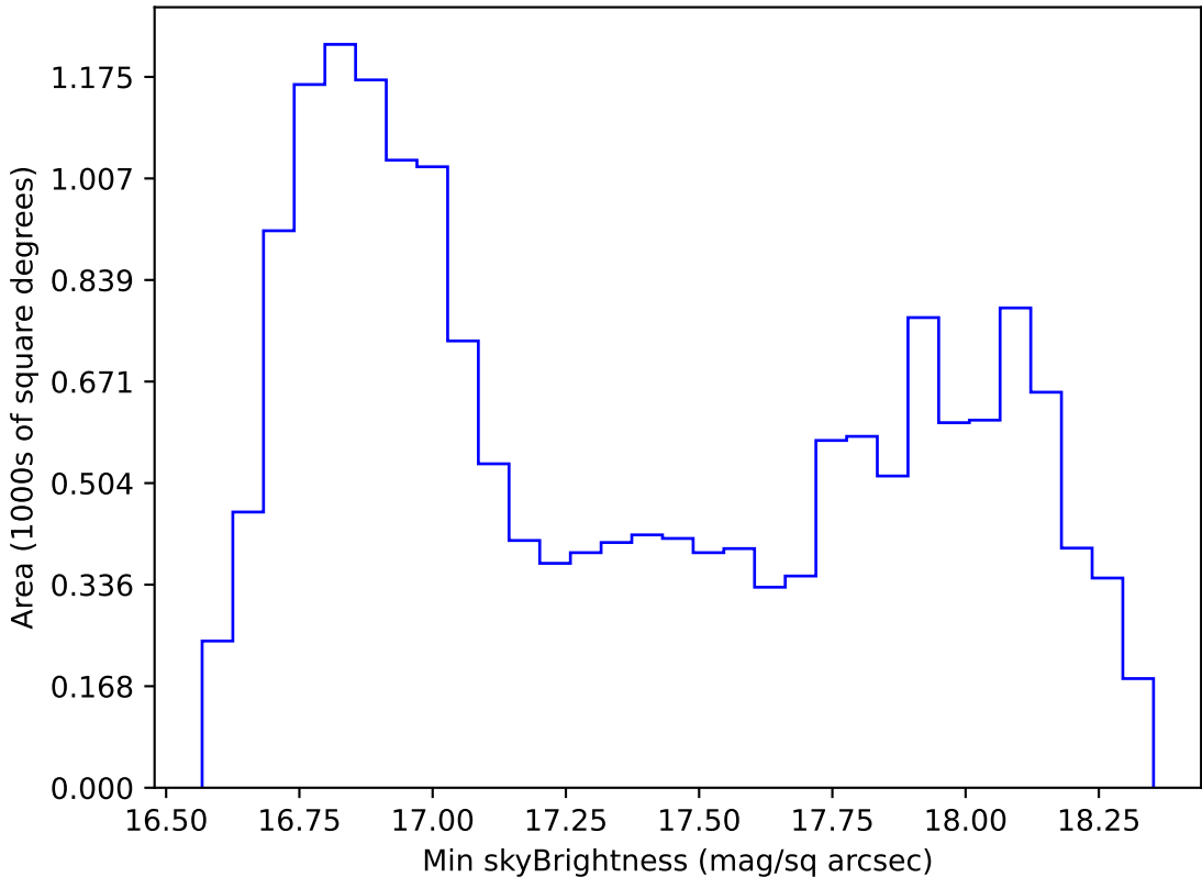
too_elab_r16_d3_gz_v3.4_10yrs WFD z band: Min skyBrightness
