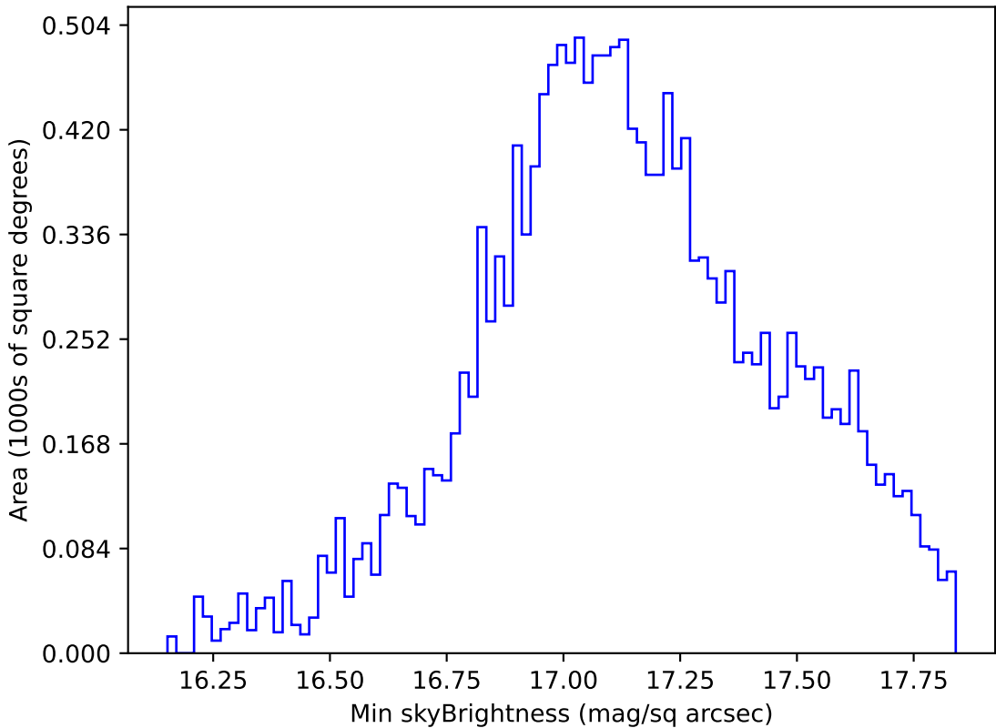
too_elab_r16_d3_gz_v3.4_10yrs WFD y band: Min skyBrightness
