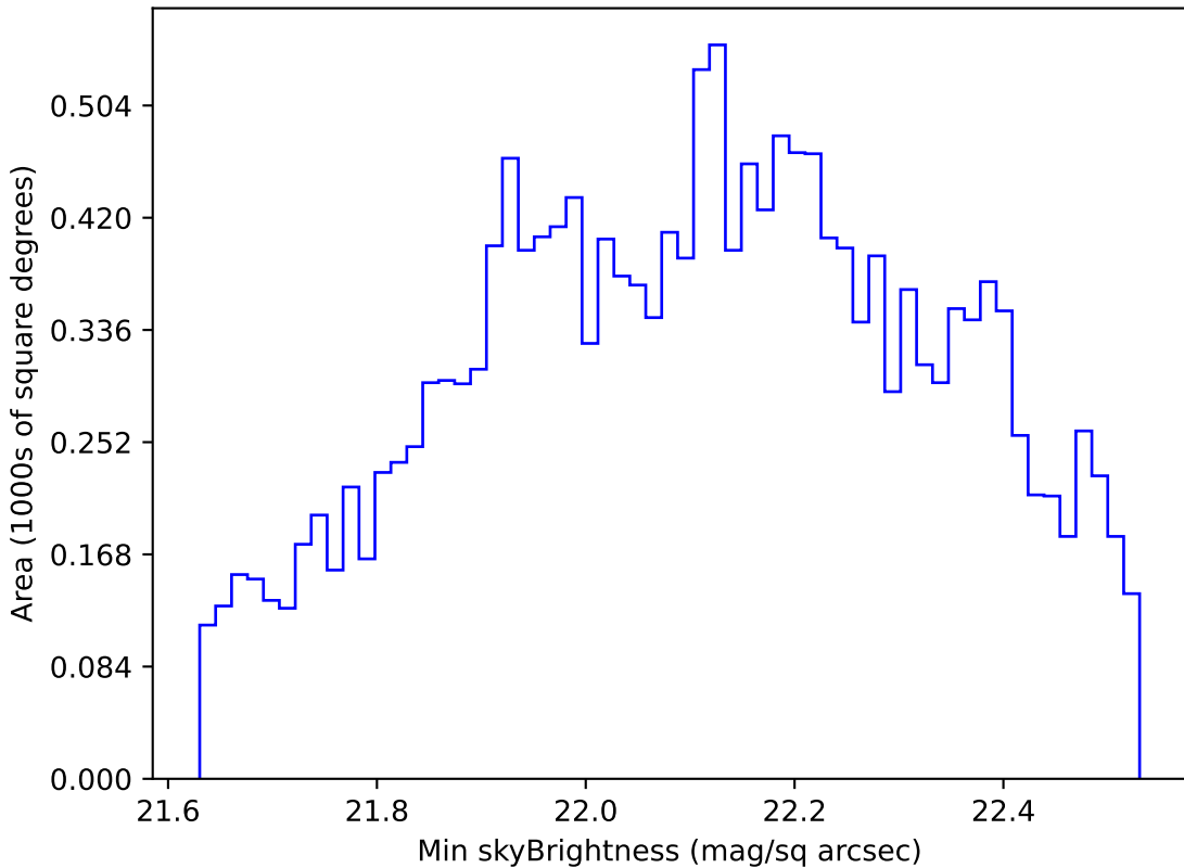
too_elab_r16_d3_gz_v3.4_10yrs WFD u band: Min skyBrightness
