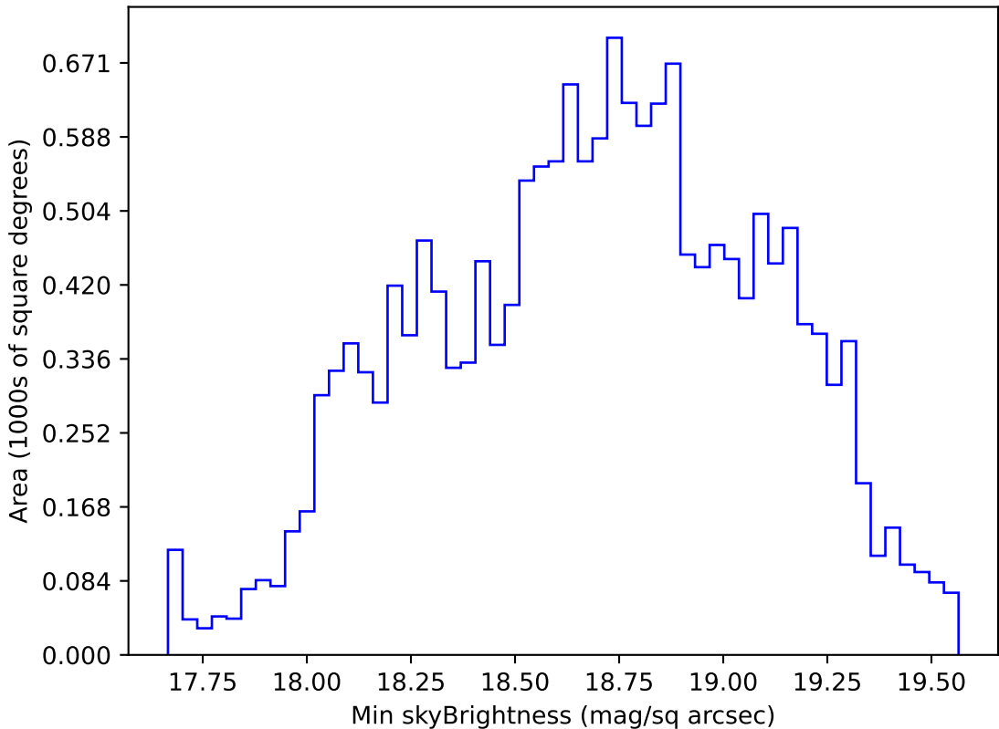
too_elab_r16_d3_gz_v3.4_10yrs WFD r band: Min skyBrightness
