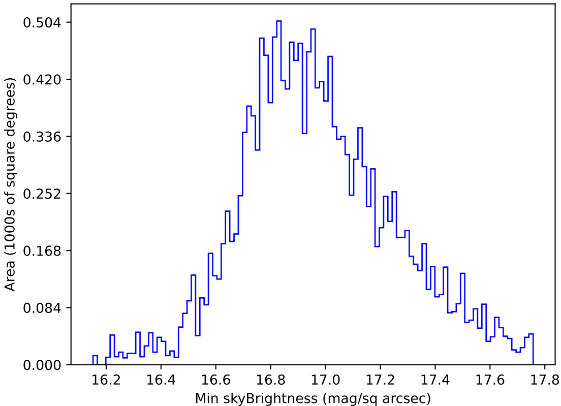
too_elab_r16_d3_gz_v3.4_10yrs WFD all bands: Min skyBrightness
