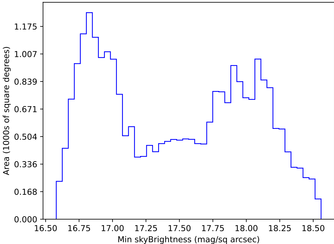
too_elab_r16_d3_gz_v3.4_10yrs All sky z band: Min skyBrightness
