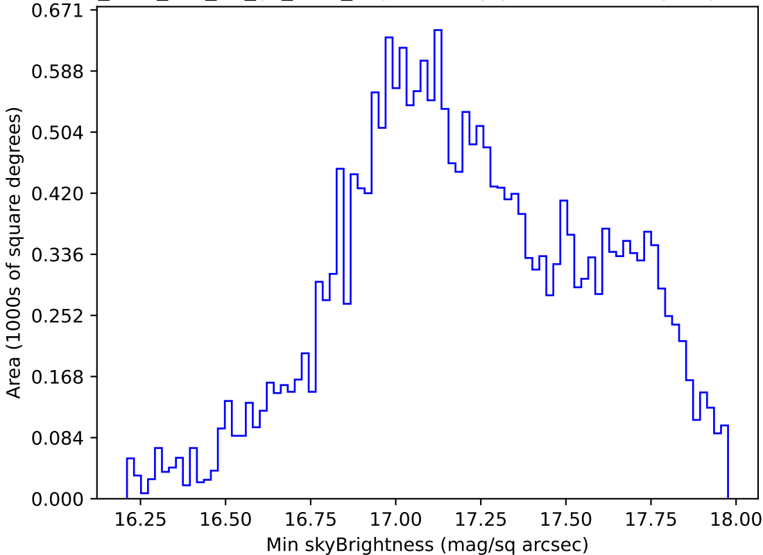
too_elab_r16_d3_gz_v3.4_10yrs All sky y band: Min skyBrightness
