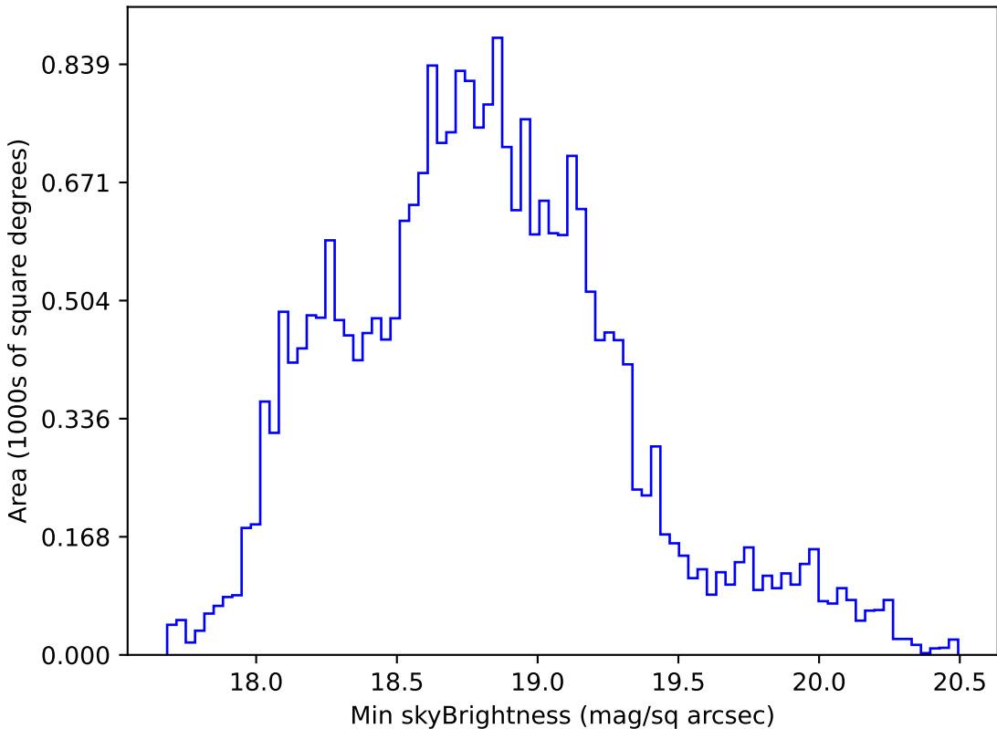
too_elab_r16_d3_gz_v3.4_10yrs All sky r band: Min skyBrightness
