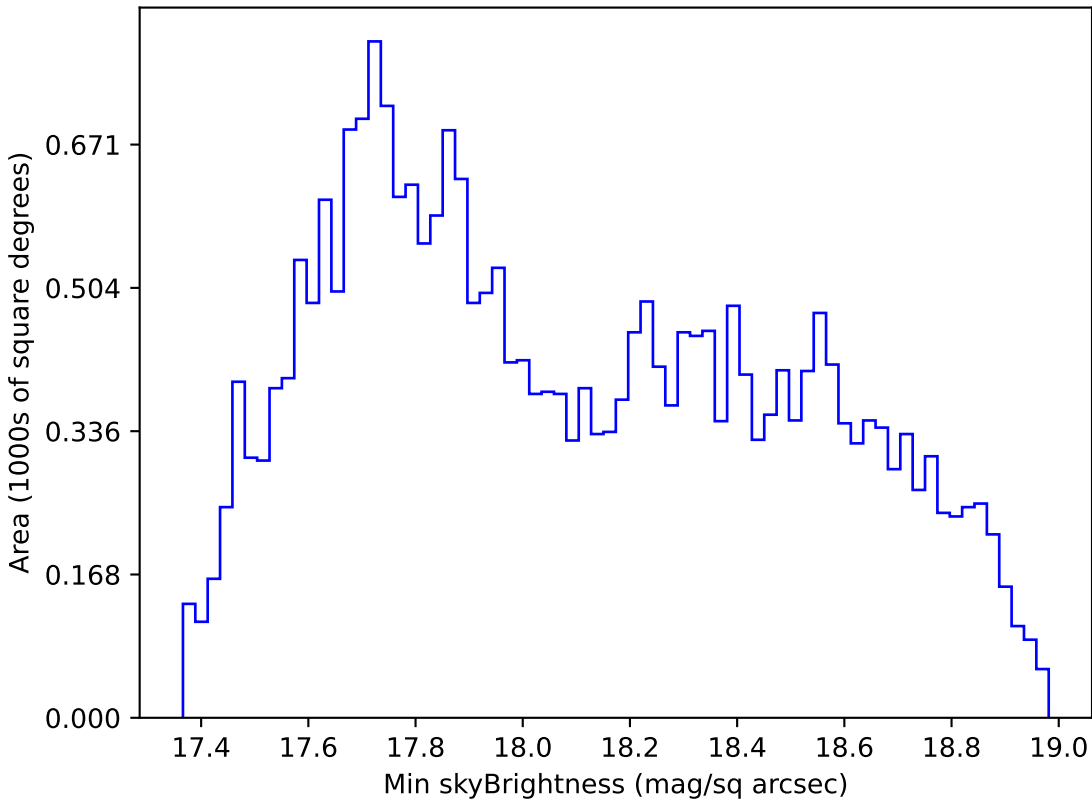
too_elab_r16_d3_gz_v3.4_10yrs All sky i band: Min skyBrightness
