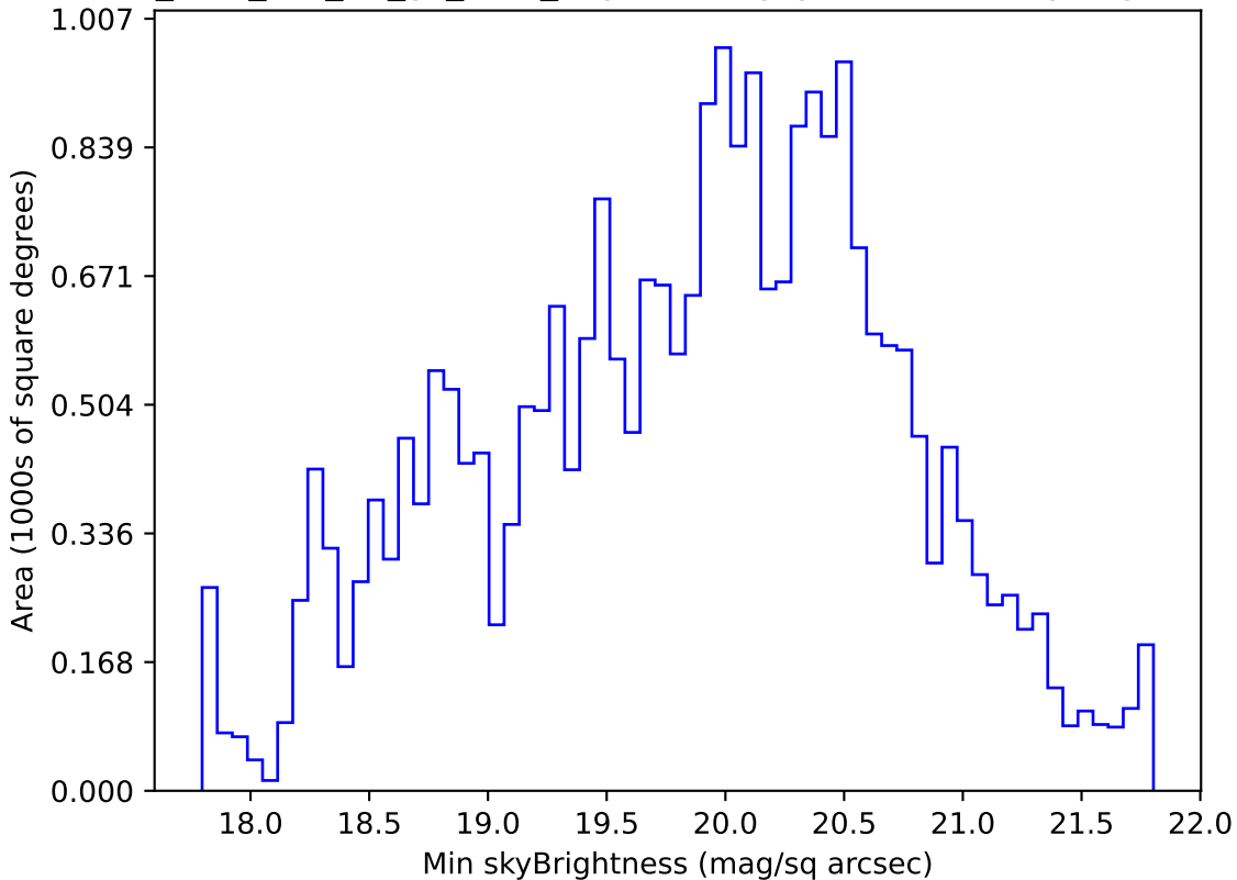
too_elab_r16_d3_gz_v3.4_10yrs All sky g band: Min skyBrightness
