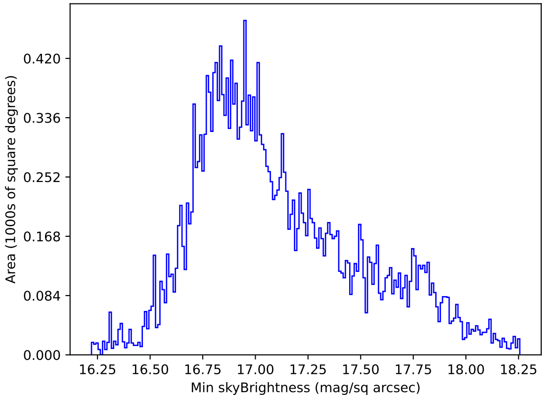
too_elab_r16_d3_gz_v3.4_10yrs All sky all bands: Min skyBrightness
