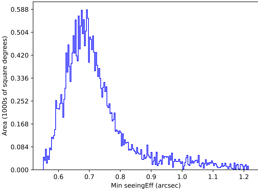
too_elab_r16_d3_gz_v3.4_10yrs Yr 1 z band: Min seeingEff
