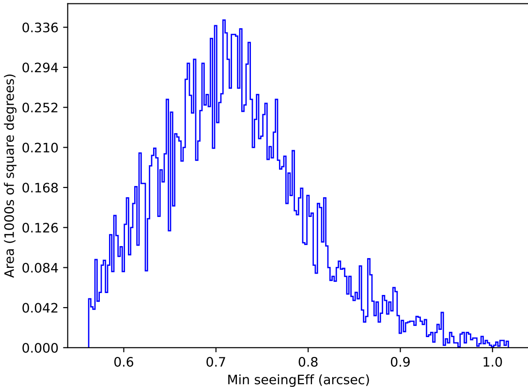
too_elab_r16_d3_gz_v3.4_10yrs Yr 1 y band: Min seeingEff
