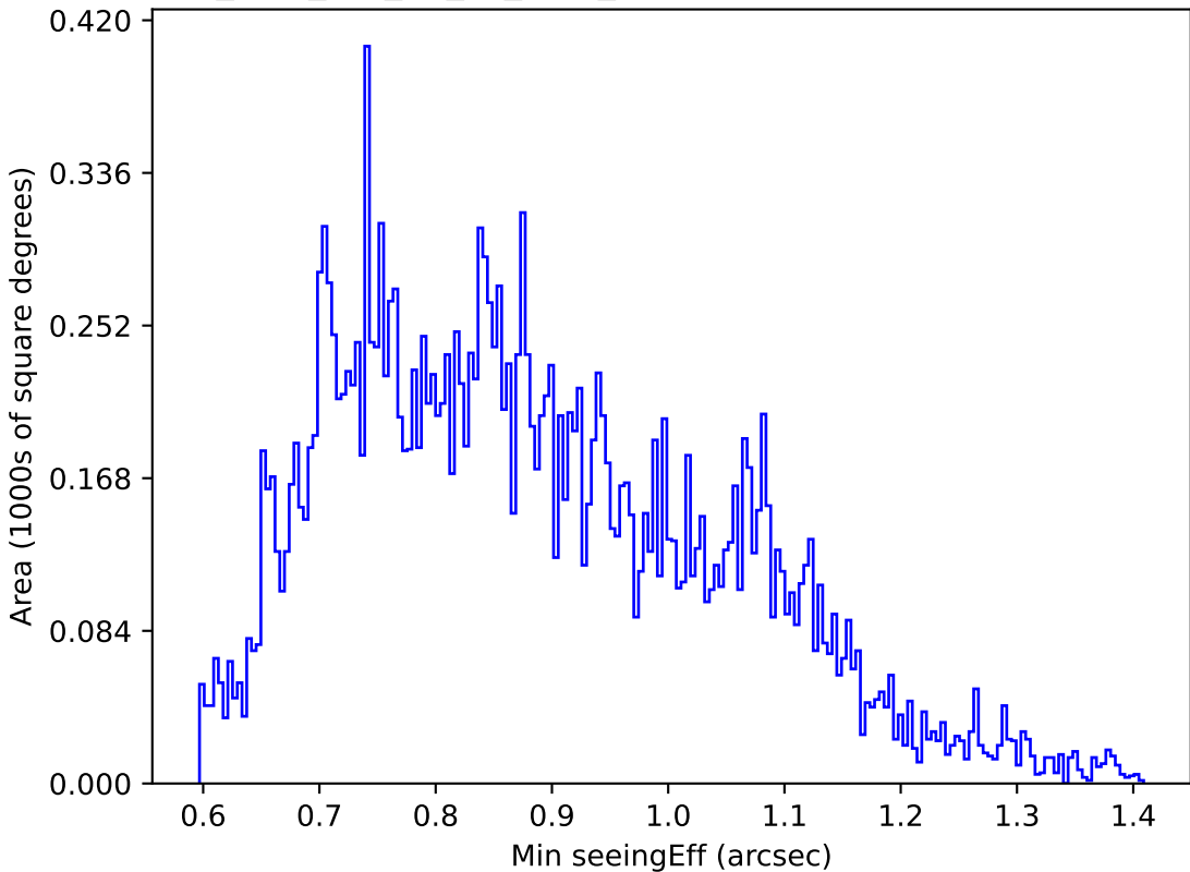
too_elab_r16_d3_gz_v3.4_10yrs Yr 1 u band: Min seeingEff
