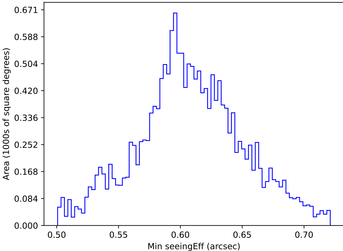
too_elab_r16_d3_gz_v3.4_10yrs WFD z band: Min seeingEff
