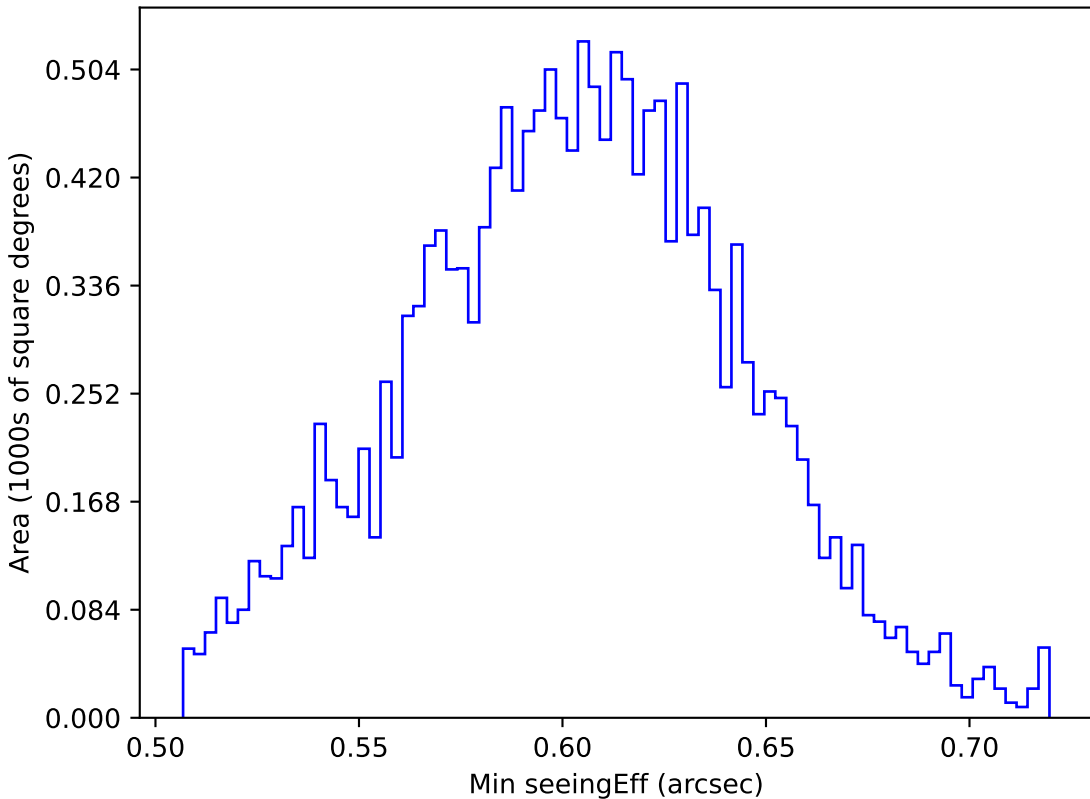
too_elab_r16_d3_gz_v3.4_10yrs WFD i band: Min seeingEff
