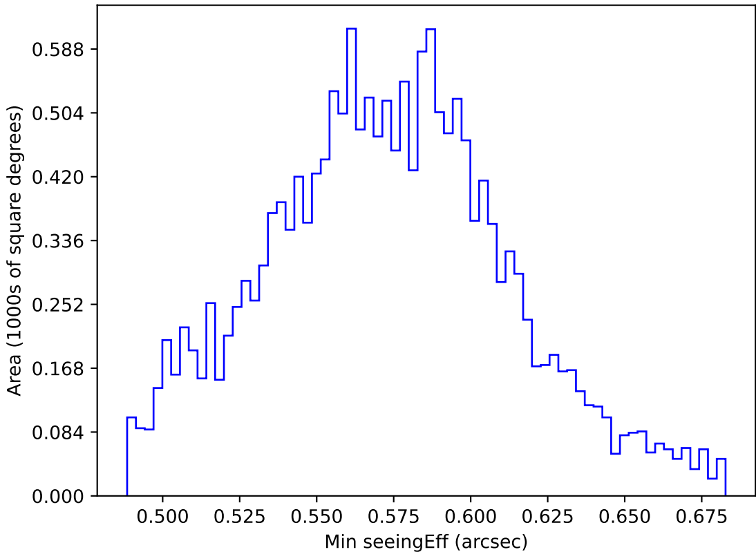
too_elab_r16_d3_gz_v3.4_10yrs WFD all bands: Min seeingEff
