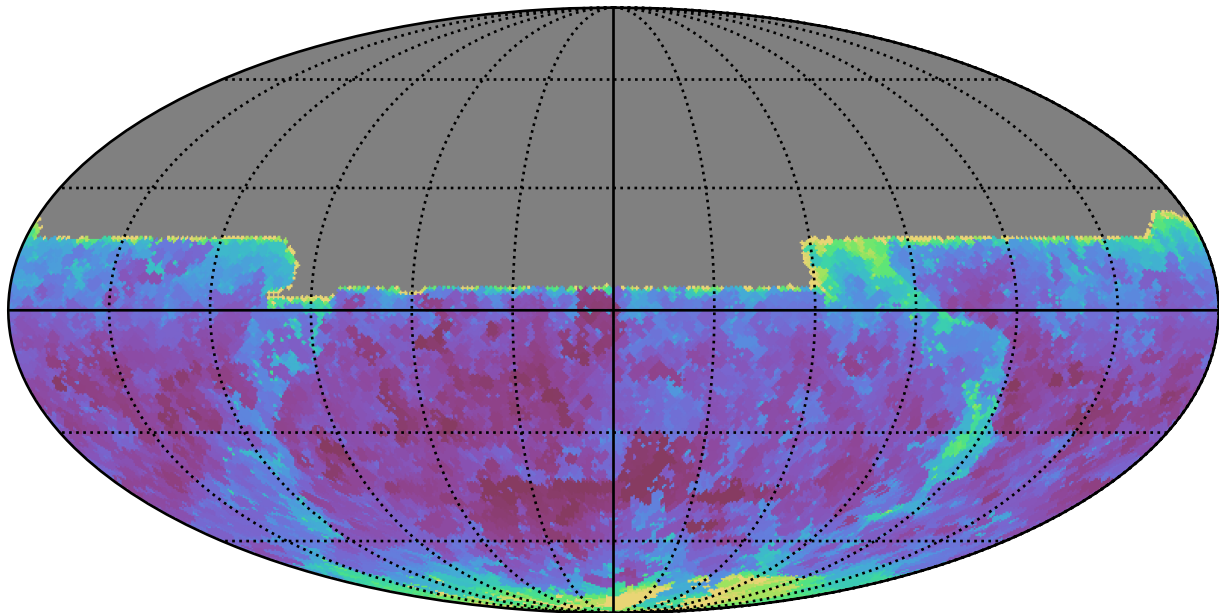
too_elab_r16_d3_gz_v3.4_10yrs All sky y band: Min seeingEff
