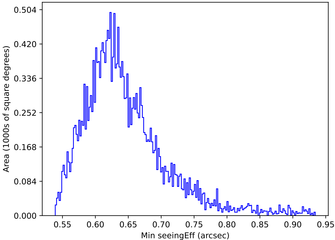
too_elab_r16_d3_gz_v3.4_10yrs All sky y band: Min seeingEff
