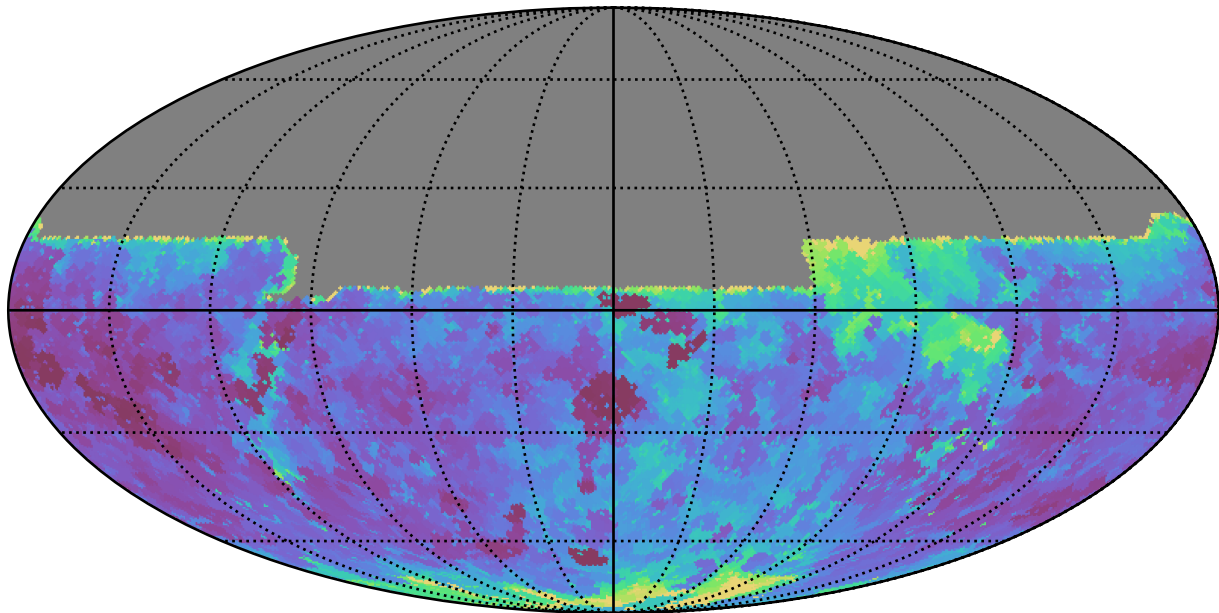
too_elab_r16_d3_gz_v3.4_10yrs All sky u band: Min seeingEff
