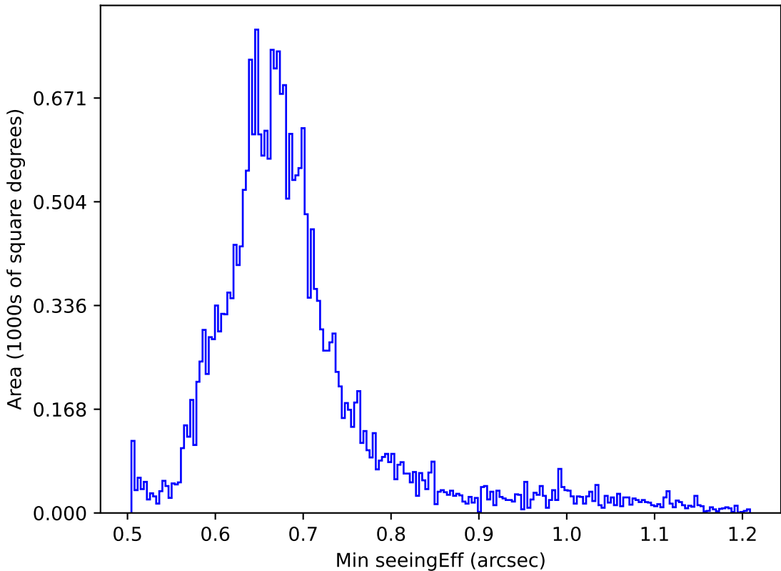
too_elab_r16_d3_gz_v3.4_10yrs All sky g band: Min seeingEff
