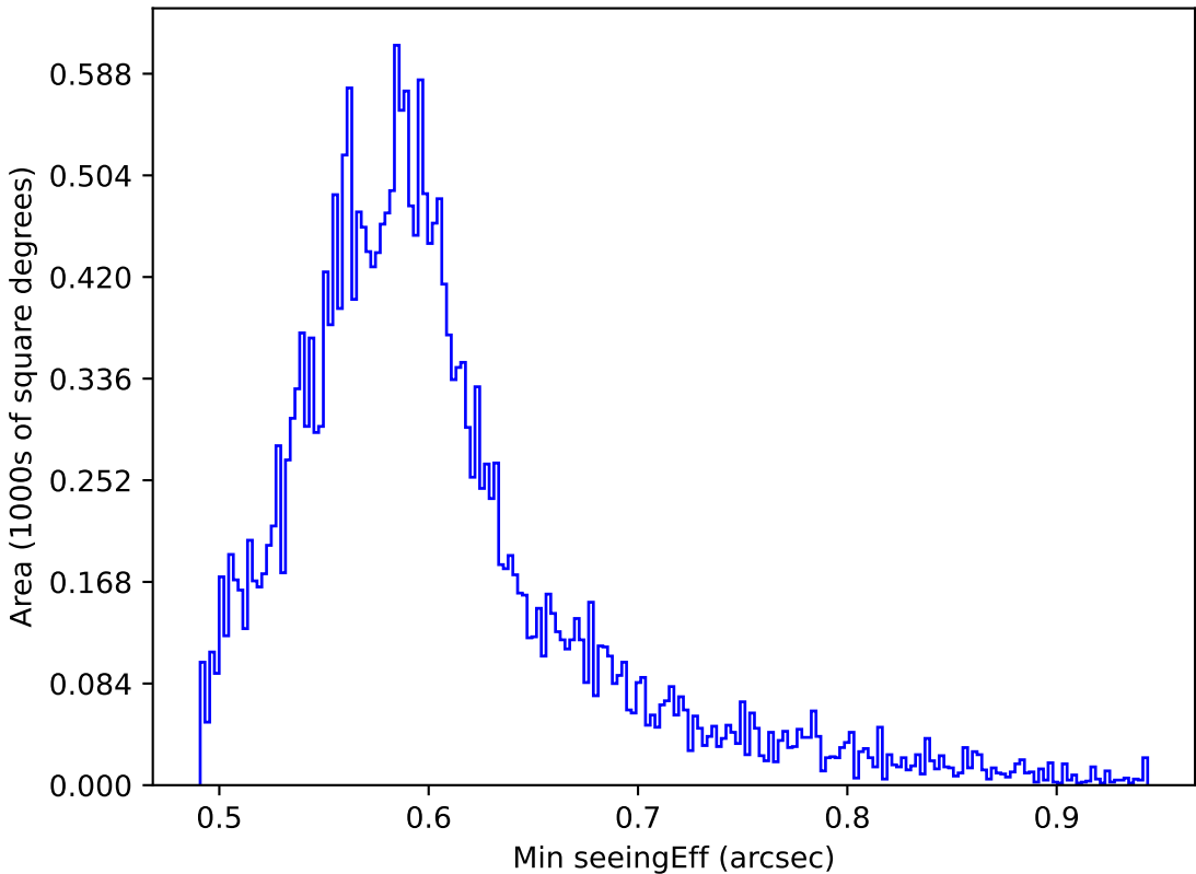
too_elab_r16_d3_gz_v3.4_10yrs All sky all bands: Min seeingEff
