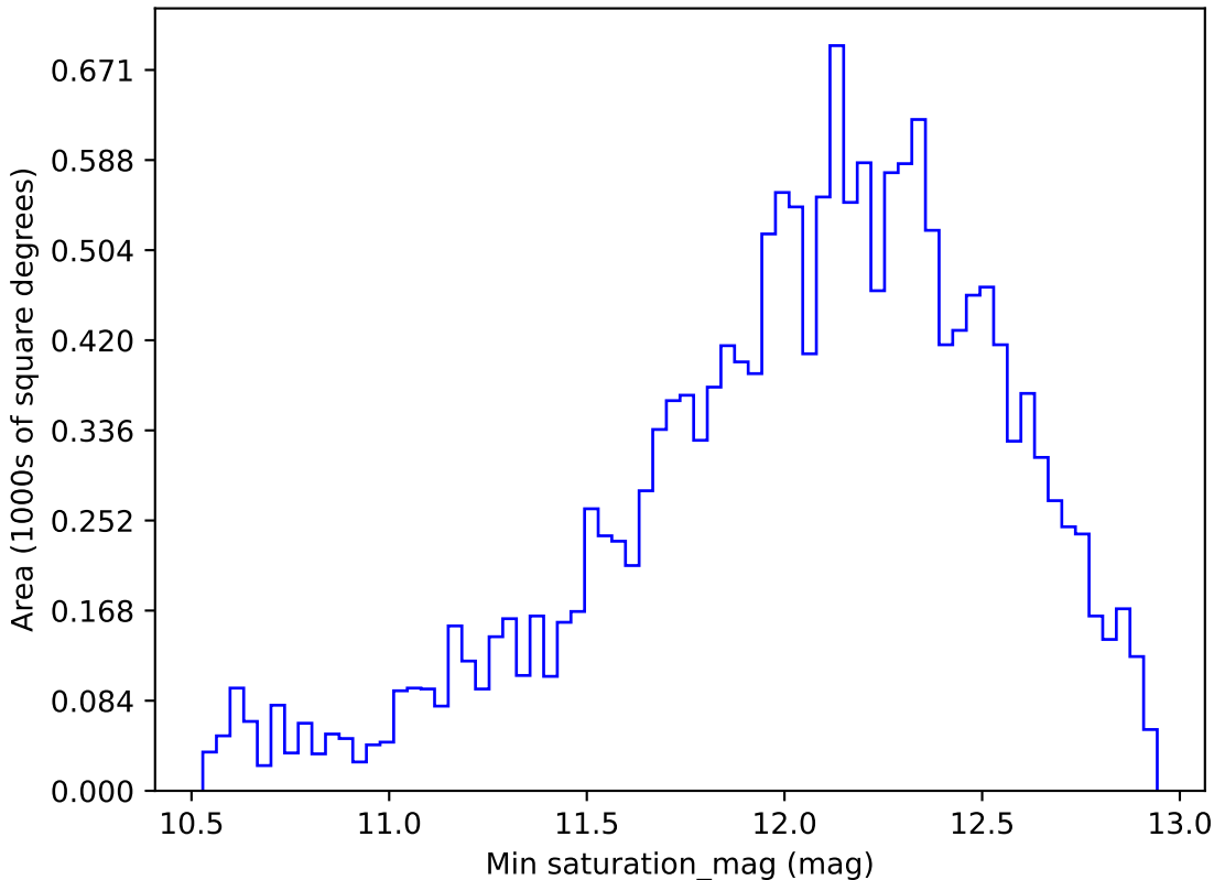
too_elab_r16_d3_gz_v3.4_10yrs WFD z band: Min saturation_mag
