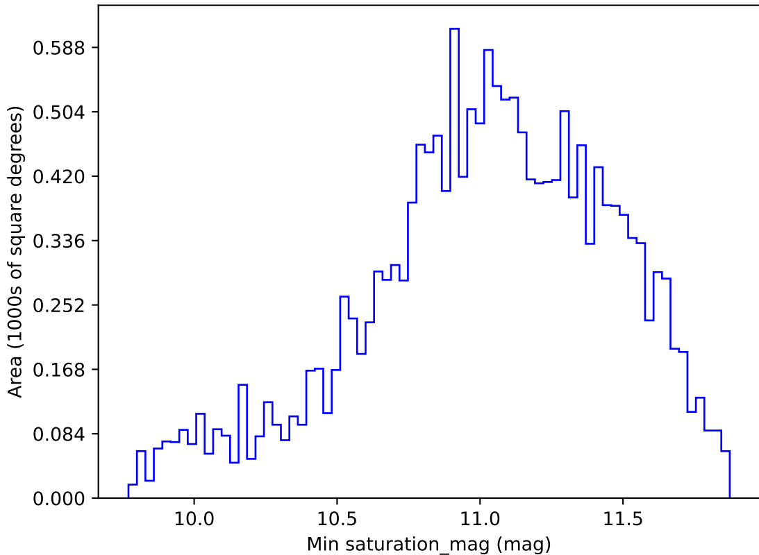
too_elab_r16_d3_gz_v3.4_10yrs WFD all bands: Min saturation_mag
