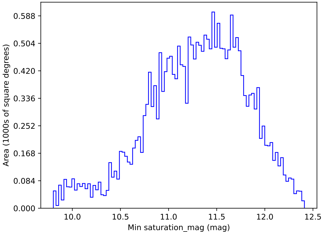
too_elab_r16_d3_gz_v3.4_10yrs All sky y band: Min saturation_mag
