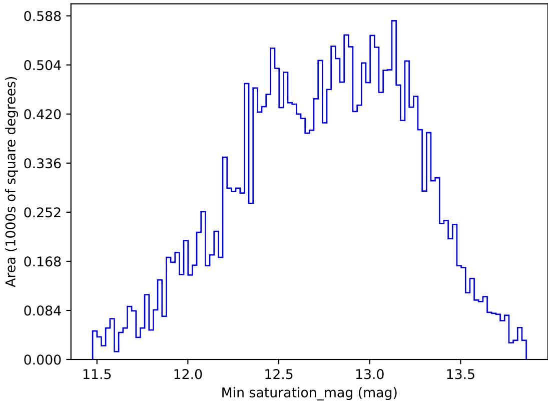
too_elab_r16_d3_gz_v3.4_10yrs All sky g band: Min saturation_mag
