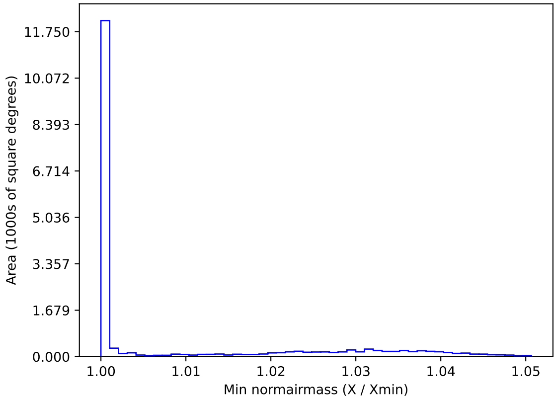
too_elab_r16_d3_gz_v3.4_10yrs WFD g band: Min normairmass
