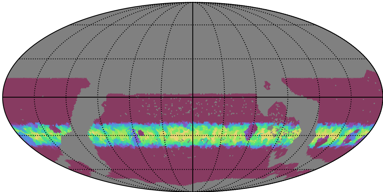
too_elab_r16_d3_gz_v3.4_10yrs WFD all bands: Min normairmass
